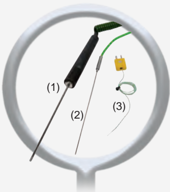
Thermocouple type K (only Fuego SCS & Fuego SCS pro, as of Serial-No. 12Zxxxxx) (1) Immersion sensor Ø 3 mm with handle, sensor length 130 mm, helix connection cable Art.-No. 8.200.240 (2) Immersion sensor Ø 1.5 mm, sensor length 150 mm, bendable, cable length 2 m Art.-No. 8.200.241 (3) Air sensor, PTFE insulated, cable length 1 m Art.-No. 8.200.242
