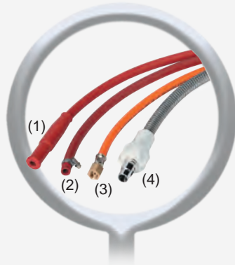
DVGW-Safety tubing (1) for push-fit connection (0.5 m) Art.-No. 6.000.102 (2) for push-fit connection, with 2 tubing clips (0.5 m) Art.-No. 6.000.101 (3) for threaded connection (0.5 m) Art.-No. 6.000.112 (4) for gas socket connection (0.5 m) Art.-No. 6.000.122 other length on demand
